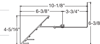
AXIFLCCKD Ceiling-to-Ceiling Knife Edge Drywall
