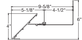
AXIFLCWKE Ceiling-to-Wall Knife Edge for Acoustical
