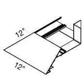
AXIFLCWKDIC Knife Edge for Drywall Ceiling-to-Wall Inside Corner
