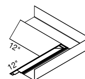
AXIFLCWKDOC Knife Edge for Drywall Ceiling-to-Wall Outside Corner
