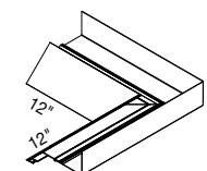
AXIFLCCKDIC Knife Edge for Drywall Ceiling-to-Ceiling Inside Corner
