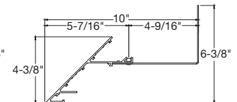
AXIFLCWKD Ceiling-to-Wall Knife Edge Drywall
