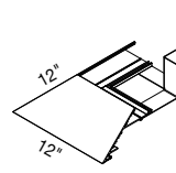
AXIFLCCKDOC Knife Edge for Drywall Ceiling-to-Ceiling Outside Corner
